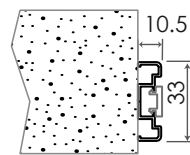
Profilo Small
