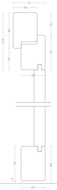
Pannello dogato Staved panel
