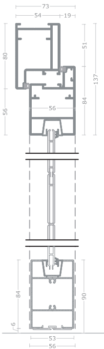
Pannello dogato Staved panel
