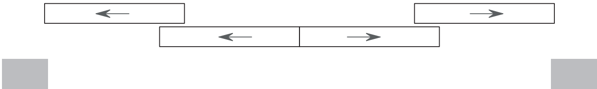
4 ante scorrevoli (anta sinistra prioritaria, vista interna) 4 sliding sashes (main left sash, internal view)
