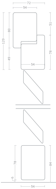
Lamella romboidale 20 Rhomboidal louver 20
