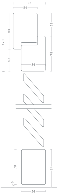
Lamella romboidale 12 Rhomboidal louver 12
