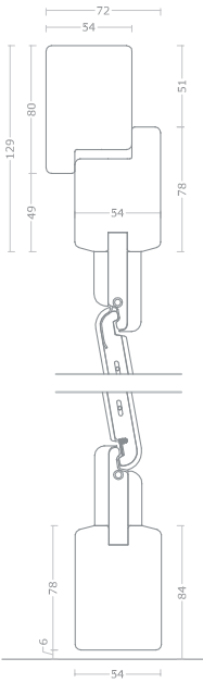
Lamella orientabile Adjustable louver
